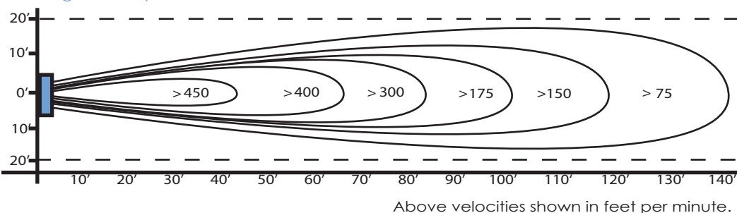
22" High Velocity Fan Air Flow Pattern
